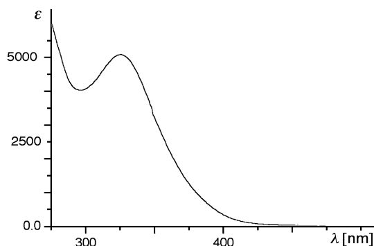
Figure 1. UV/Vis absorption spectrum of compound 13 in CHCl 3 at room temperature.
