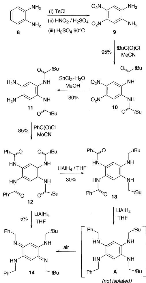
Scheme 1. Synthesis of molecules 13 and 14 .
