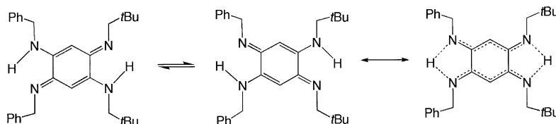
Scheme 2. Tautomeric equilibrium of 14 in solution.
