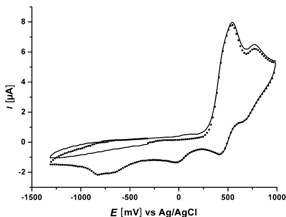
Figure 2. Cyclic voltammogram of compound 13 in \text{CH}_2\text{Cl}_2 [ 0.1 \text{ M N}(\text{nBu})_4\text{PF}_6 ] starting in oxidation (—) and in reduction (---).
